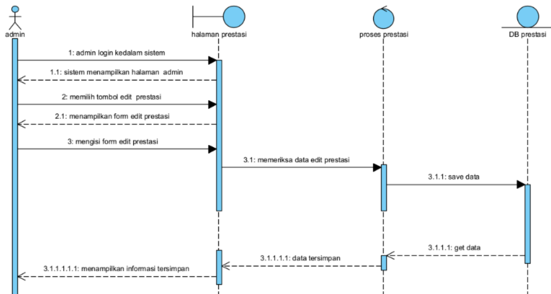
Gambar 25 Sequence Diagram mengedit prestasi
