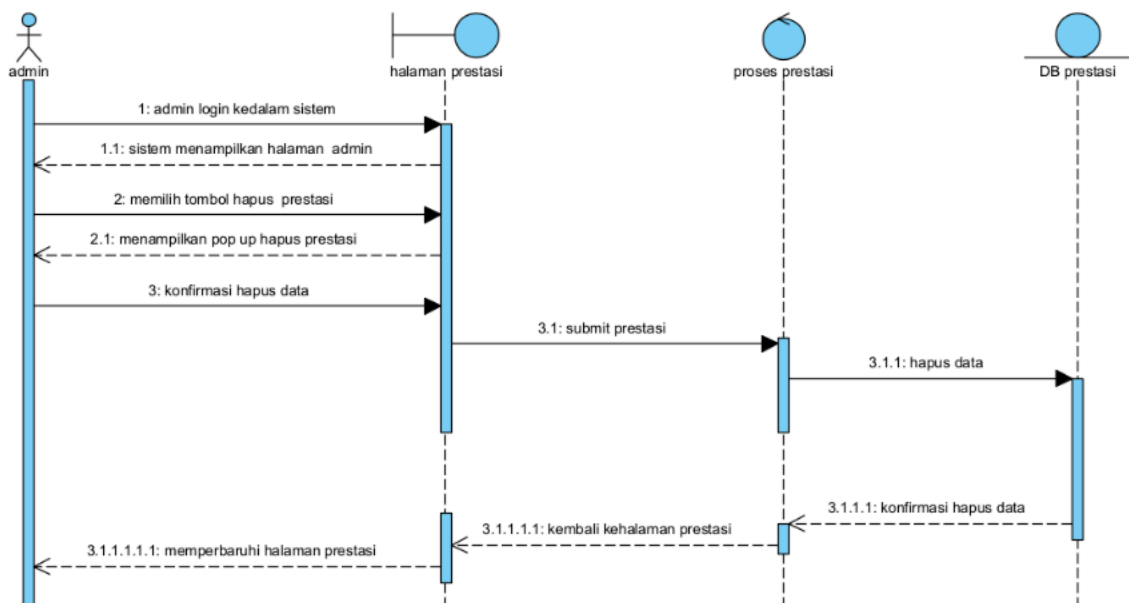
Gambar 28 Sequence diagram menghapus prestasi
