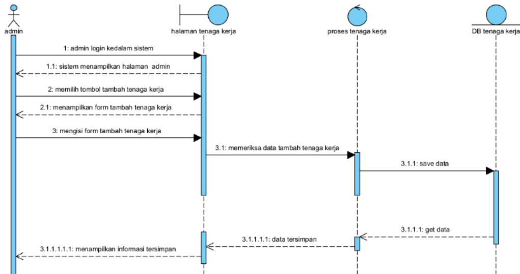
Gambar 19 Sequence Diagram menambah tenaga kerja
