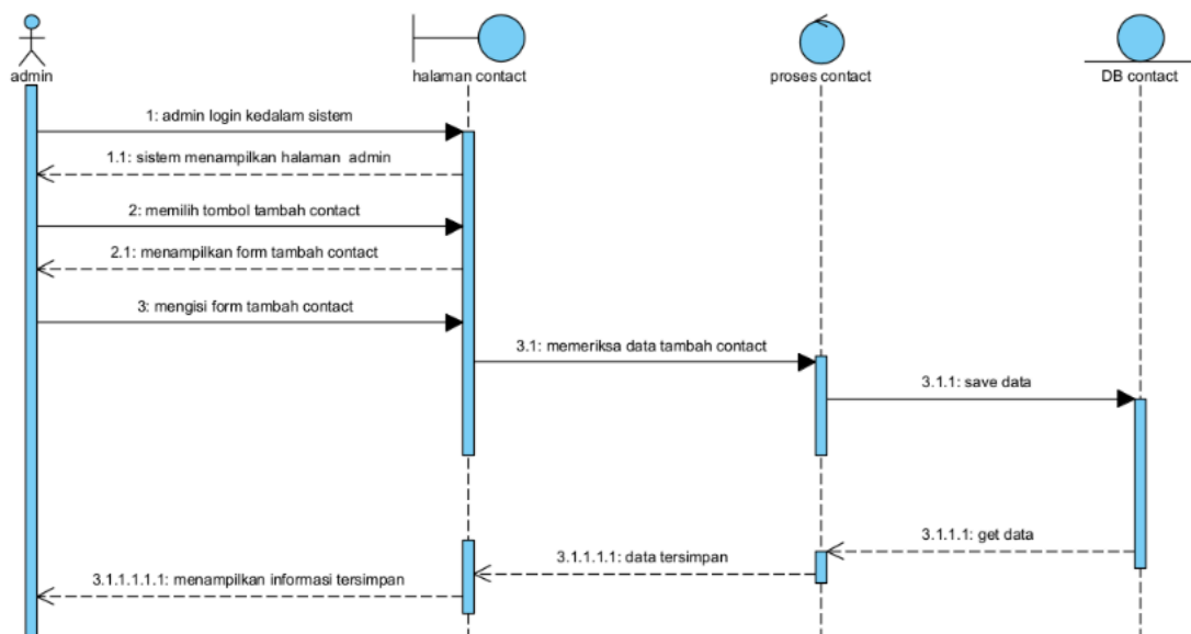
Gambar 18 Sequence Diagram menambah contact
