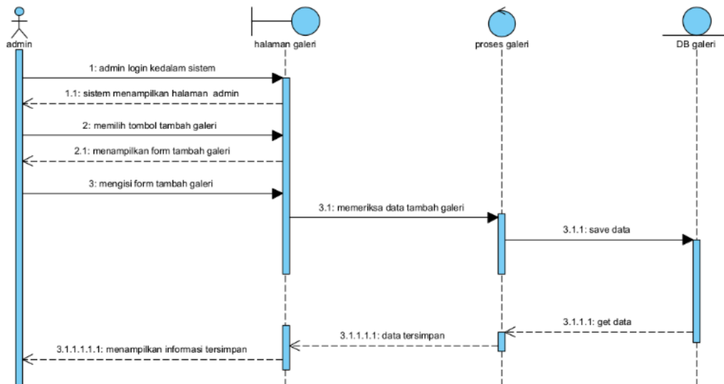
Gambar 16 Sequence Diagram menambah galeri
