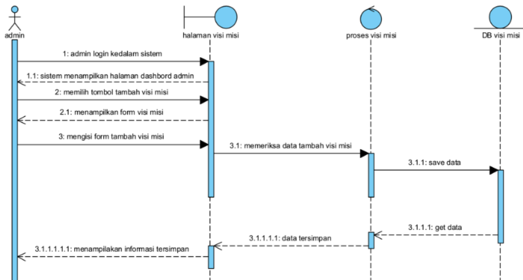
Gambar 14 Sequence Diagram menambah visi-misi
