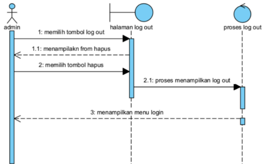
Gambar 35 Sequence Diagram log out
