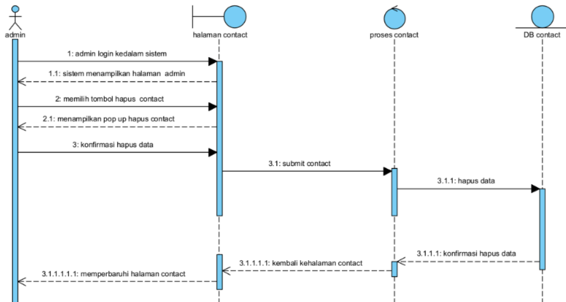
Gambar 32 Sequence Diagram menghapus contact
