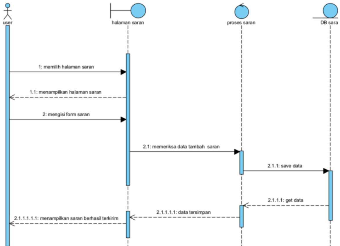
Gambar 20 Sequence Diagram menambah saran guest
