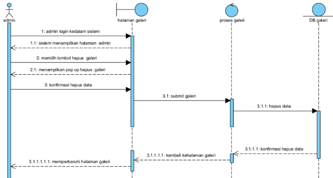
Gambar 29 Sequence diagram menghapus galeri
