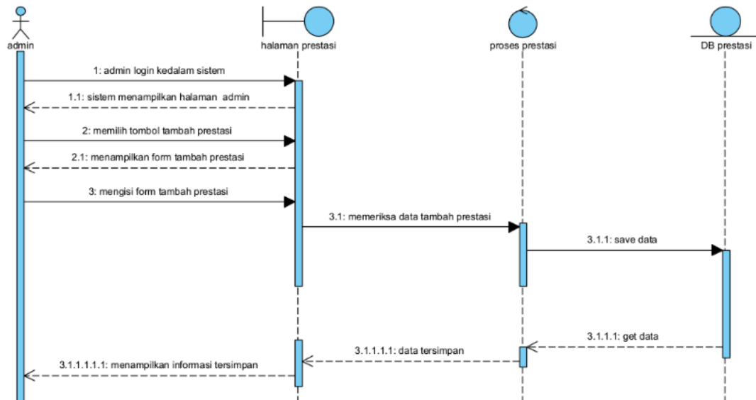
Gambar 15 Sequence Diagram menambah prestasi
