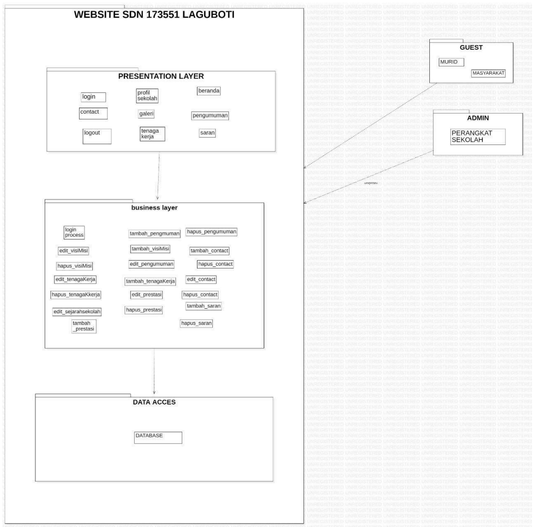
Gambar 3 Package Diagram Website SD Negeri 173551 Laguboti
