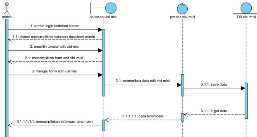
Gambar 23 Sequence Diagram mengedit visi misi
