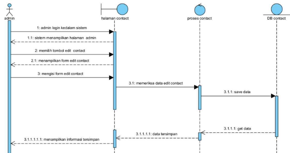
Gambar 22 Sequence Diagram mengedit contact
