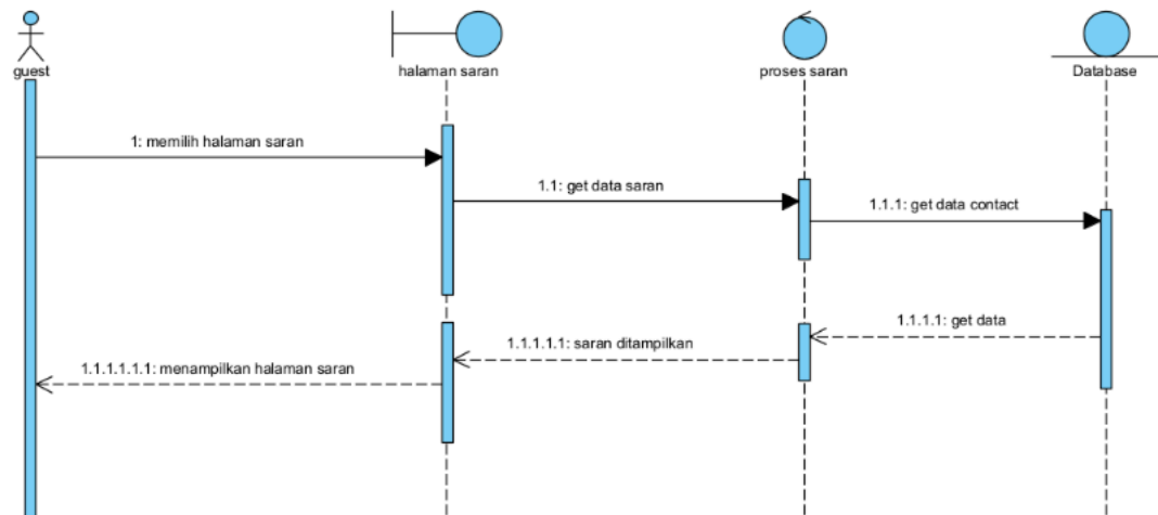
Gambar 13 Sequence Diagram Melihat saran
